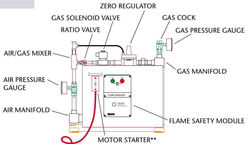
Photo Shows One Burner Flame Treating System
