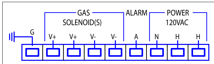
Wiring Diagram
